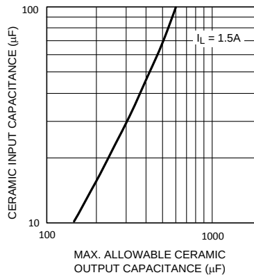
Figure 19. Maximum Ceramic Output Capacitance vs Ceramic Input Capacitance
